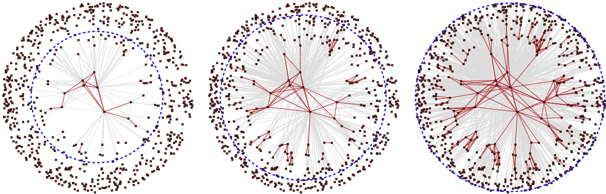
Figure 4. Evolution of a Milne network at three different proper times. The dashed blue circles represent the expanding horizons of the central observer. The grey and red links show directed and bi-directed (reciprocal) connections. The central observer and all its connections are suppressed.
