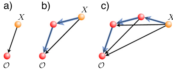
Figure 1. Direct versus indirect causal relations. Black edges show the direct causal relations between observers. In (b) and (c) the blue paths are indirect causal relations between observers X and O .
