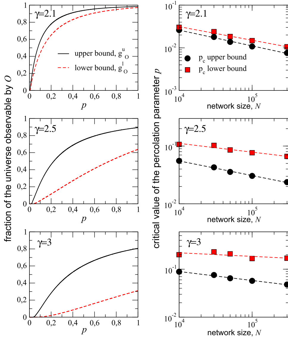
Figure 6. Bond percolation simulations of imperfect-communication networks. The left column shows the upper and lower bounds g_O^{u,l}(p) for the fraction of nodes causally connected to O for different values of \gamma and N = 3 \times 10^5 . The right column shows the critical values p_c^{u,l}(N) for the same bounds, measured as the value of p that maximizes the susceptibilities \xi^{u,l} in equation (18). The dashed lines are power law fits p_c^{u,l}(N) \sim N^{-1/\nu} with exponents 1/\nu = 0.3(7) , 0.3(2) for \gamma = 2.1 , 1/\nu = 0.2(5) , 0.1(5) for \gamma = 2.5 , and 1/\nu = 0.1(8) , 0.0(7) for \gamma = 3 .
