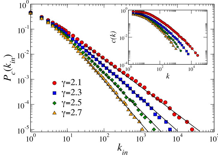
Figure 5. Complementary cumulative in-degree distribution P_c(k_{in}) = \sum_{k_{in}' \geq k_{in}} P(k_{in}') in simulated Milne networks with exponents \gamma = 2.1, 2.3, 2.5, 2.7 grown up to N = 10^5 nodes. The solid lines are power laws with the same exponents. Inset: degree-dependent clustering coefficient for the undirected versions of the same networks. The average clustering coefficients excluding nodes of degree 1 are \bar{C} = 0.67, 0.47, 0.41, 0.38 for \gamma = 2.1, 2.3, 2.5, 2.7 , respectively. The networks are disassortative, meaning that the correlations of degrees of connected nodes (not shown) are negative, due to structural constraints imposed by the scale-free degree distribution [13].
