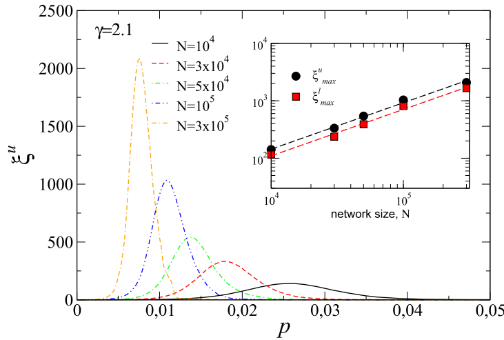
Figure 7. Percolation susceptibility of the upper bound \xi^u equation (18) as a function of p for different network sizes and \gamma = 2.1 (results for other values of \gamma are qualitatively similar). For all values of \gamma < 3 , \xi^u and \xi^l show a peak that moves to the left as the system size increases. At the same time, the maximum value of \xi^u and \xi^l diverges as a function of N as \xi_{max}^{u,l} \sim N^{\gamma'/\nu} . Dashed lines in the inset are power law fits with exponents \gamma'/\nu = 0.8(0) .
