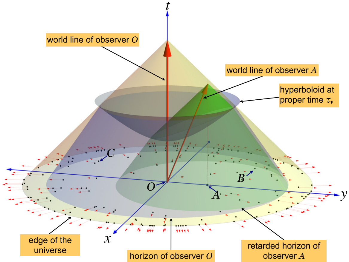
Figure 2. Milne universe with overlapping horizons as seen by observer O at proper time \tau > \tau_v . The horizontal plane is the (x, y) plane in a (2 + 1) -dimensional Minkowski spacetime. The vertical axis t is the proper time of observer O , who is at rest in the cosmic fluid, \chi = 0 and x = y = 0 . At cosmic time \tau = 0 , all particles are at the origin of this Minkowski spacetime and start moving away from O at velocities v , according to equation (4). Points and arrows in the (x, y) plane represent the position and velocity of such particles at proper time \tau , as measured by O . The ‘edge of the universe’ corresponds to particles receding from O at the speed of light. Thus, this edge is a circle of radius R_{edge} = \tau centered at O . Observer O does not observe all particles within this edge because particles are ‘lit,’ not at \tau = 0 , but at \tau_v > 0 . These events lie on the invariant hyperboloid t^2 = \tau_v^2 + x^2 + y^2 , which is shown in blue. The horizon of any given observer is then induced by the intersection of the past light cone with this hyperboloid, and defines the maximum speed of a particle within the horizon. In particular, the radius of O ’s horizon in the (x, y) plane is R_{horizon} = \tau [1 - (\tau_v/\tau)] / [1 + (\tau_v/\tau)] ( \tau_v = 1.5 and \tau = 5 in the figure). The thick red arrows show the world lines of stationary observers O and A . Observer A is at rest at radial coordinate \chi = \text{const} . The retarded horizon of observer A at proper time \tau_\chi is induced by the intersection of A ’s past light cone with the blue hyperboloid. Projected into the (x, y) plane, this retarded horizon encompasses all observers that can causally influence O indirectly via A (figure 1). Observer O has incoming connections from observers A , B , and C because they all lie within O ’s horizon. Observer A has incoming connections from O and B , but not from C , who is outside A ’s horizon.
