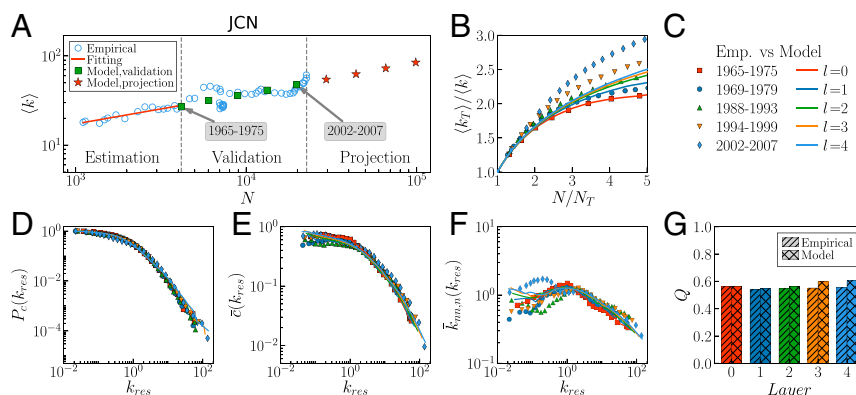
Fig. 4. The GBG model predicts the self-similar evolution of real networks. (A) Evolution of the average degree \langle k \rangle vs. network size N . The estimation, validation, and projection sections are separated by vertical dashed lines. Blue circles, green squares, and red stars represent empirical data, validation points, and projection from the model, respectively. The data in the estimation section are used to find values of a (see details in SI Appendix, section VI ). The branching rate, b , is fixed to 1.5, and the corresponding value of a is 1.415 ( SI Appendix, Fig. S20 ). For validation purposes, we grow the network from 1965 to 1975 using GBG and compare the resulting networks with empirical (Emp.) snapshots of the same size. The equivalence between given snapshots of the real JCN and the networks generated by GBG is stated in C. In D–G, we show a comparison of the topological properties of simulated and empirical networks. (B) Local rich-club effect. (D) Complementary cumulative distribution of rescaled degrees. (E) Degree-dependent clustering coefficient over rescaled-degree classes. (F) Degree-degree correlations. (G) The modularity Q .
